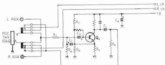
Fig. 7 Microphone circuitry
