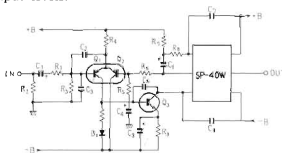
Fig. 10 Power amplifier circuitry
